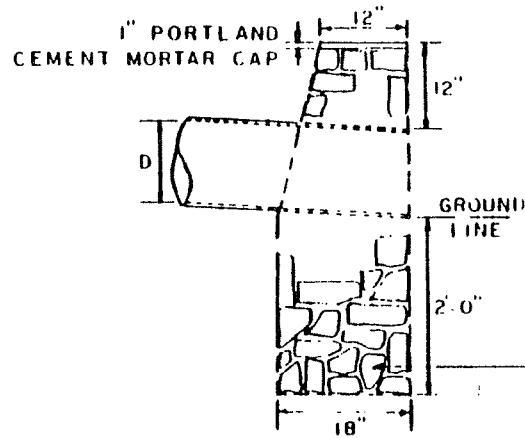
END ELEVATIONS
